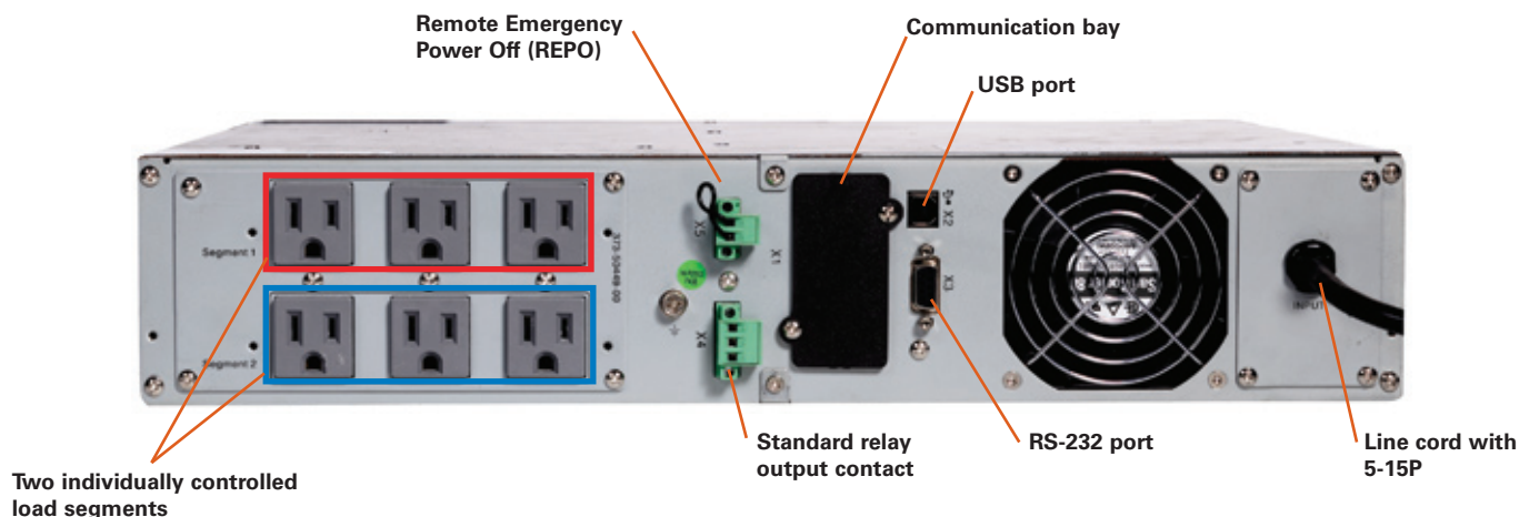
UPS rear panel (PW9130L1500R-XL2U)
