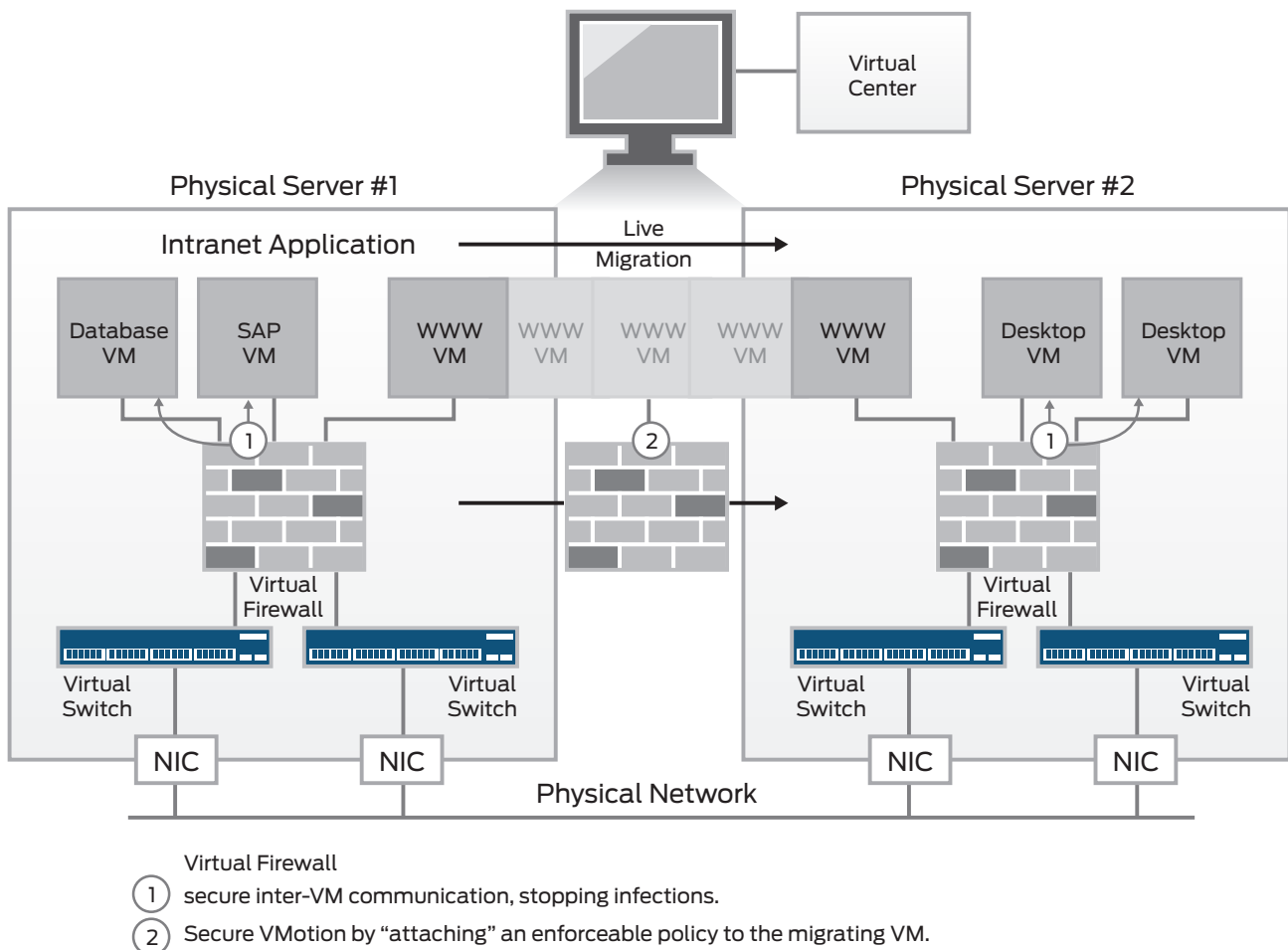
Figure 2: vGW secures highly dynamic VMs through change and motion.
