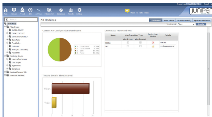
Figure 3: The vGW antivirus allows for on-demand and on-access scanning of VMs and files.
